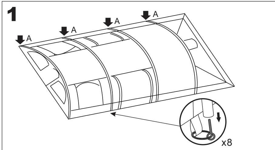
Inner Tent (already hang on fly during packing)
